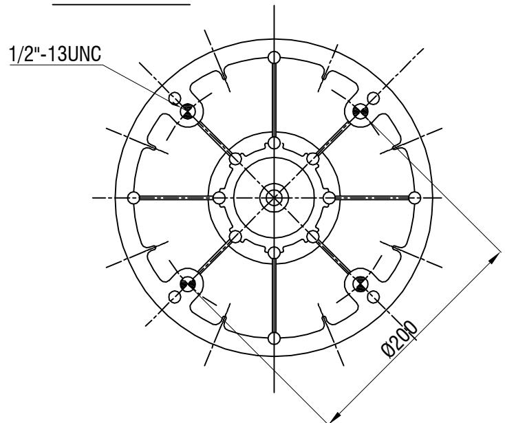
BOTTOM VIEW
