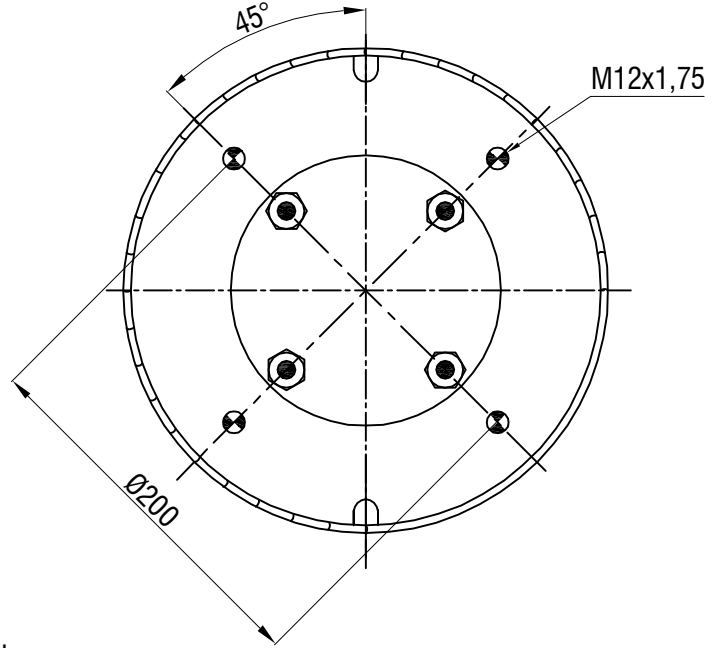
BOTTOM VIEW
